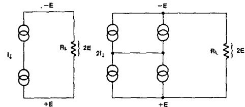
Fig. 9 Adding Two Current Sources to Double the Current
