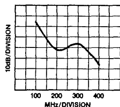
Fig. 13 Harmonic Performance of the Circuit Shown in Figure 11 at 1 dB Gain Compression
