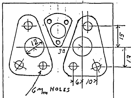
CATHODE CAPACITOR PLATES
