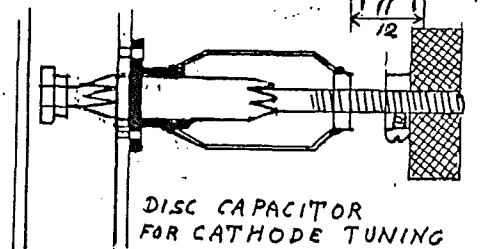
CATHODE CAPACITOR PLATES
