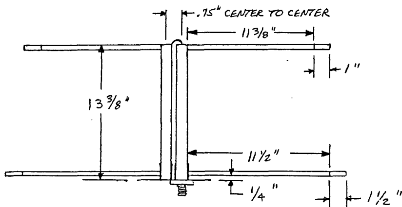
70 cm DIPOLE FEED
