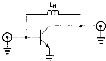
Fig. 10 AC Equivalent Circuit Neutralized Device
