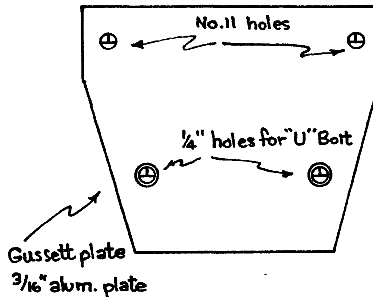
Figure 5 - Element Loop Yagi for 1296 MHz - Spacing drawing
