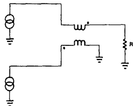
Fig. 6 Balun Combiner
