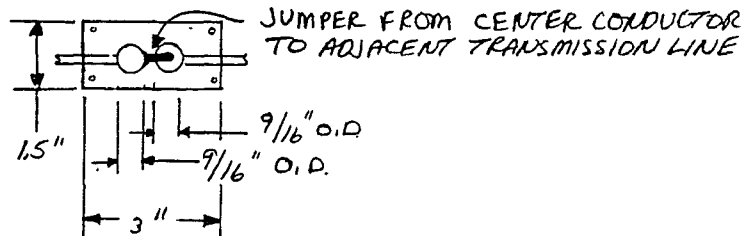
70 cm DIPOLE FEED
