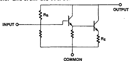
Fig. 1 RB - Shunt Feedback Resistor RE - Series Feedback Resistor
