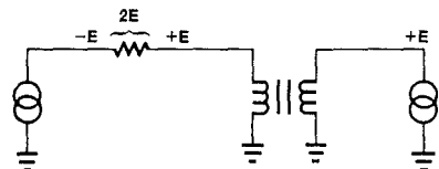
Fig. 7 Conventional Transformer Configuration
