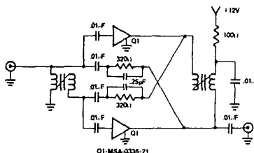
Fig. 11 Unilateralized Push-Pull Circuit
