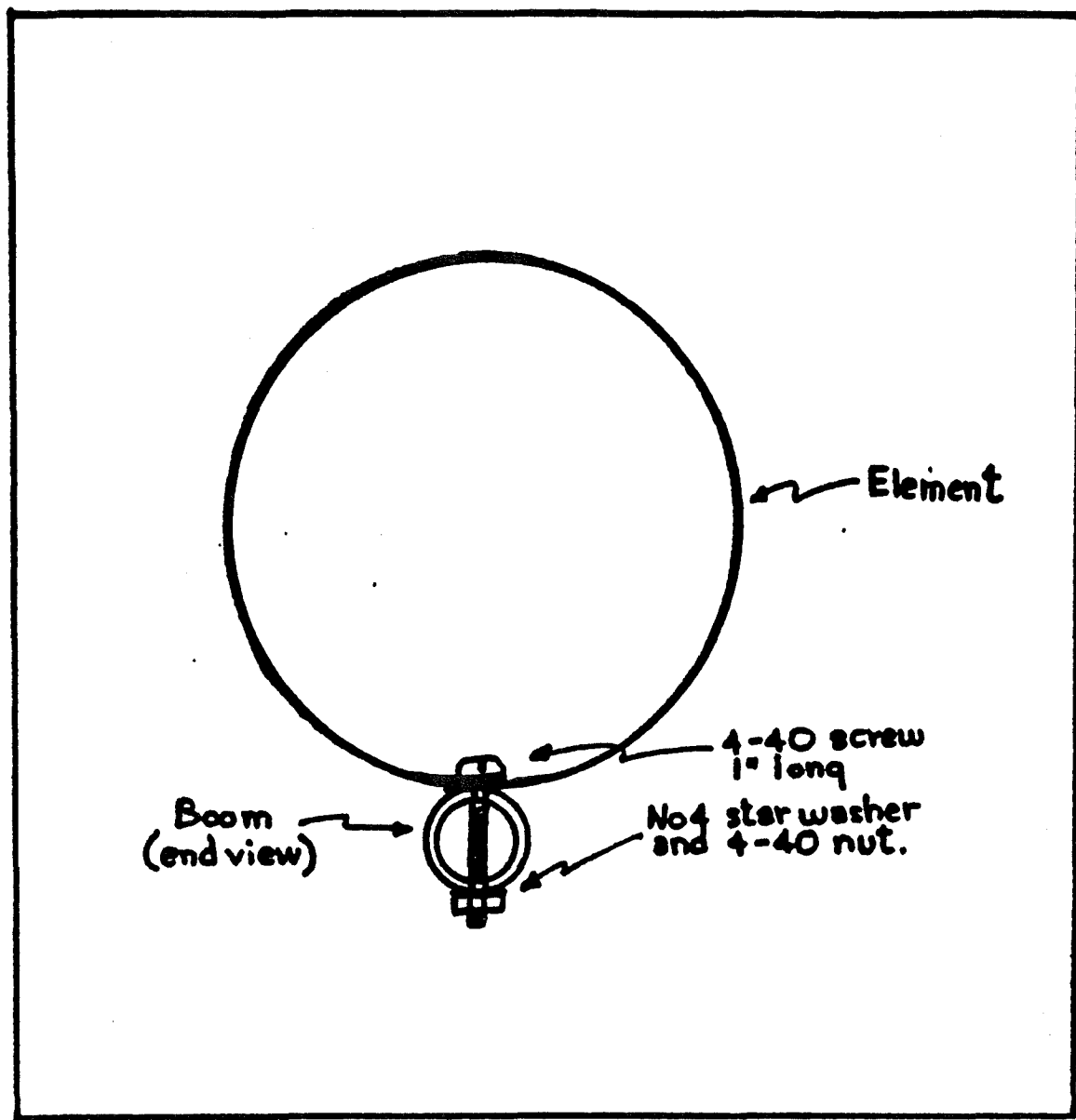
Figure 3 - How the elements are mounted
