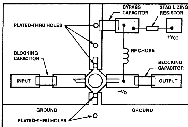
TYPICAL -21 AND -22 MODEL MOUNTING CONFIGURATION
